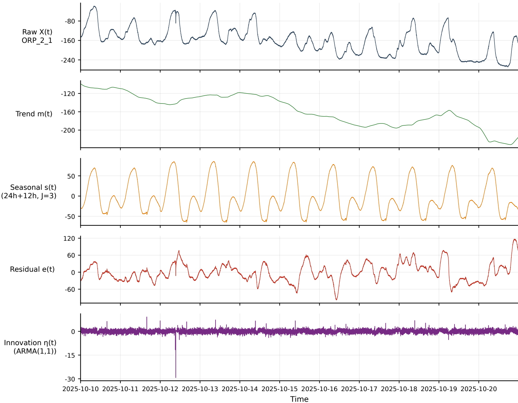
Multi-scale decomposition — ORP_2_1 (anaerobic, min) [2025-10-10~2025-10-20]
